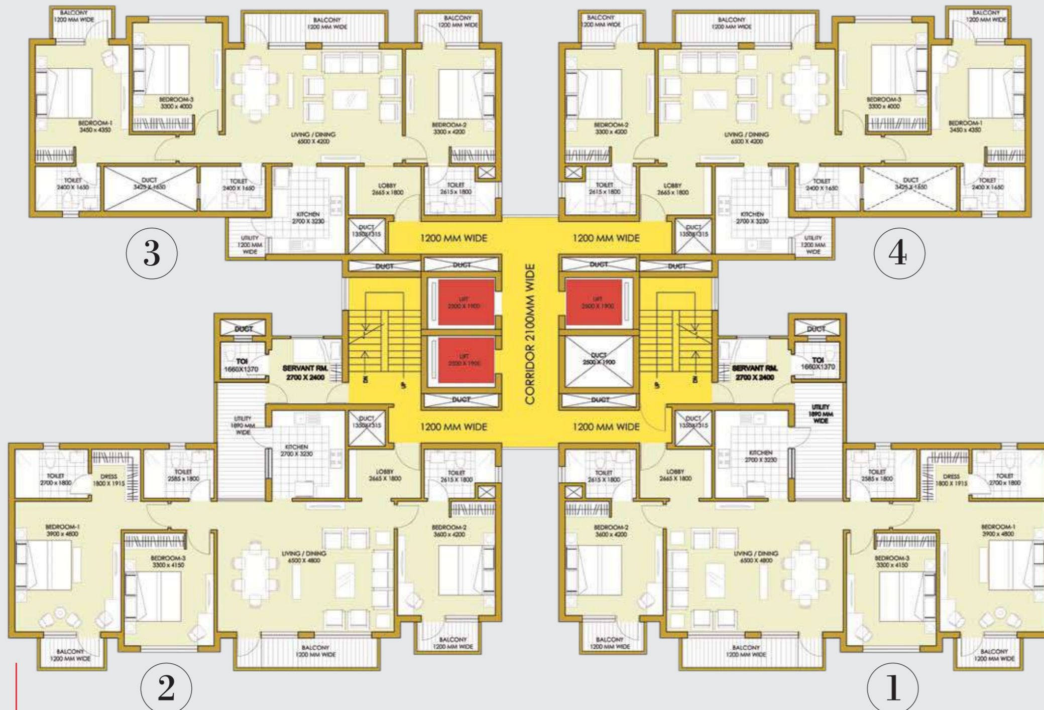
Floor Plan - Type C
